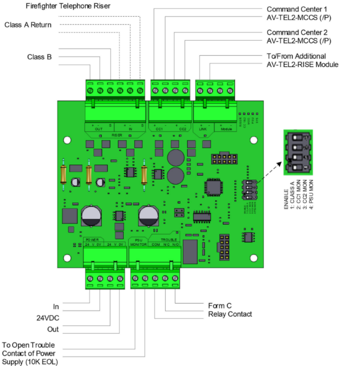
AV-TEL2-RISE Module Wiring and DIP switch
